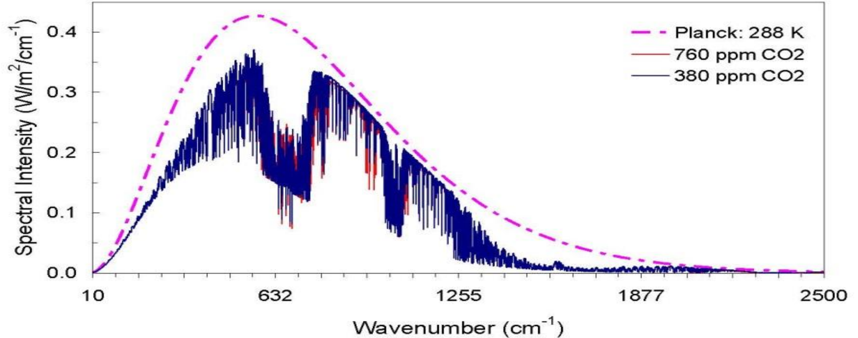
Global upwelling radiation in the atmosphere for the GH-gases \text{H}_2\text{O} , \text{CO}_2 , \text{O}_3 and \text{CH}_4 at T=288\text{K}
