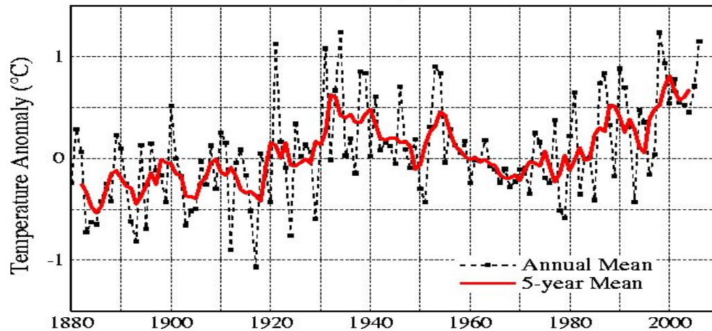
U.S. Temperature
